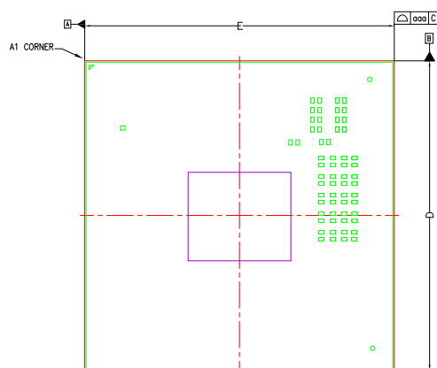
TOP VIEW (1)
